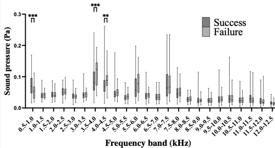
Fig. 2 The sound pressure (Pa) in different frequency bands (kHz) of successful and unsuccessful press-fit fixation.
