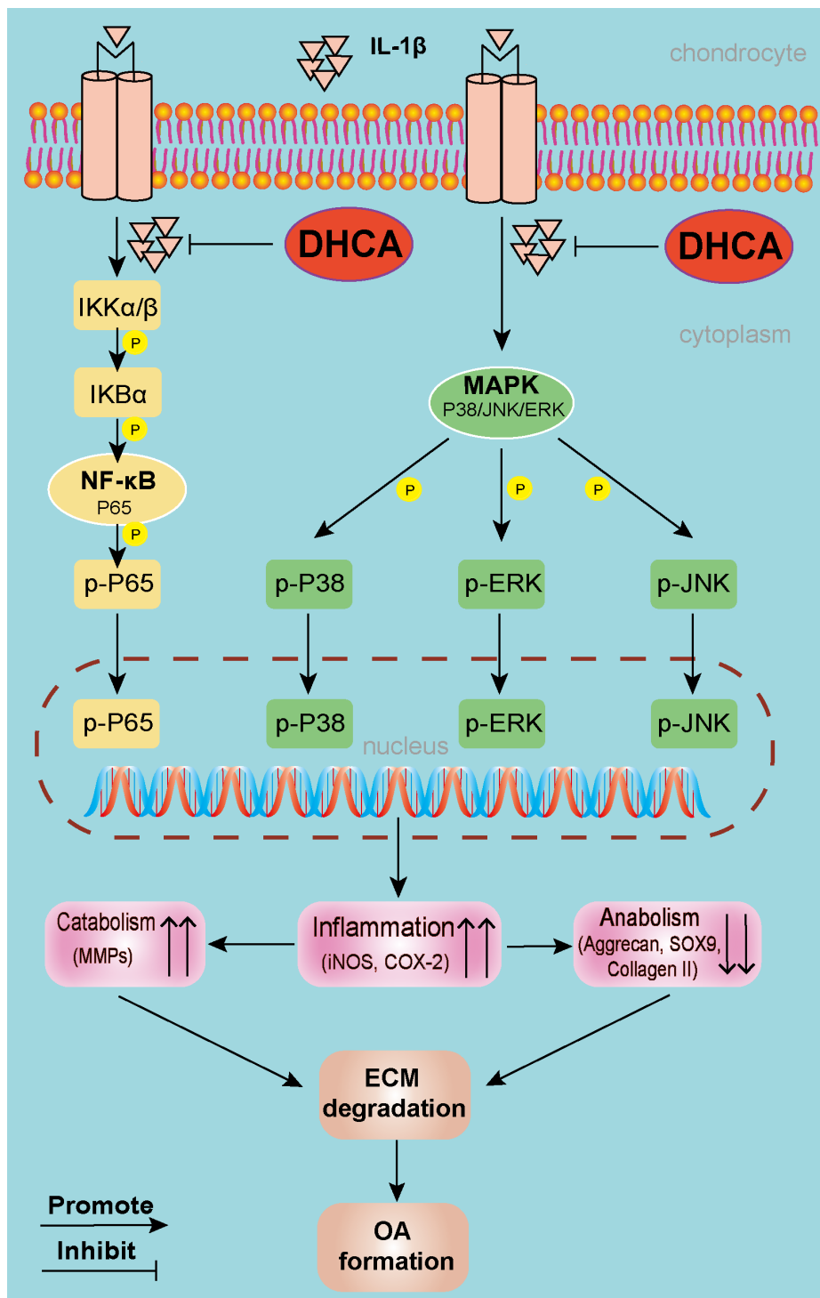
Fig a. Schematic diagram of dihydrocaffeic acid (DHCA) improving in mouse osteoarthritis (OA). Interleukin-1 \beta (IL-1 \beta ) was employed to establish OA chondrocytes in vitro. The enhanced catabolism, increased inflammation, and inhibited anabolism induced by IL-1 \beta were reversed by DHCA.
